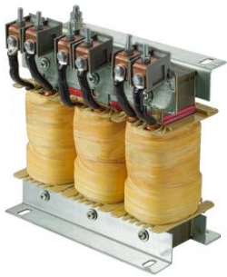
THREE-PHASE
